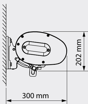
tak installation
