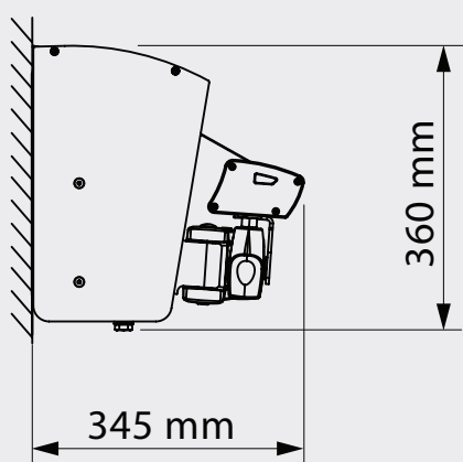
wall installation
