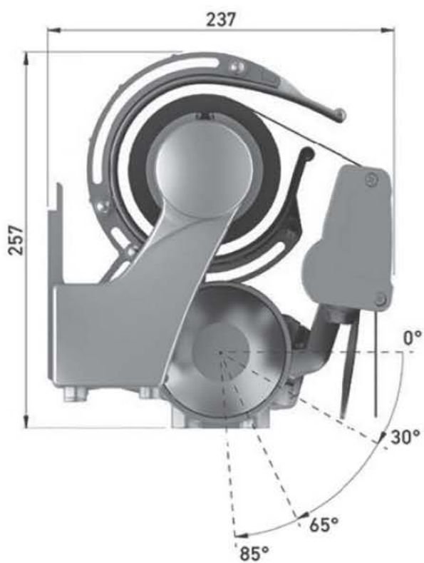
Wall installation
