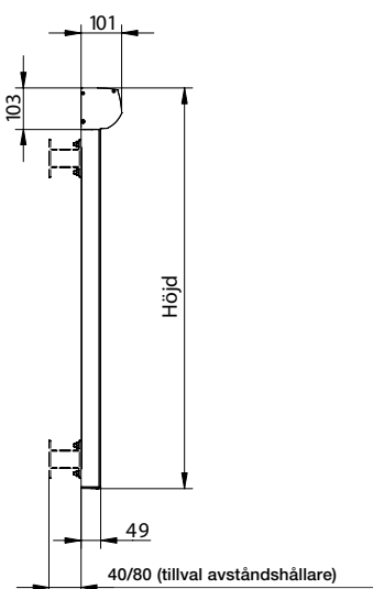
Skruvskena (standard)
